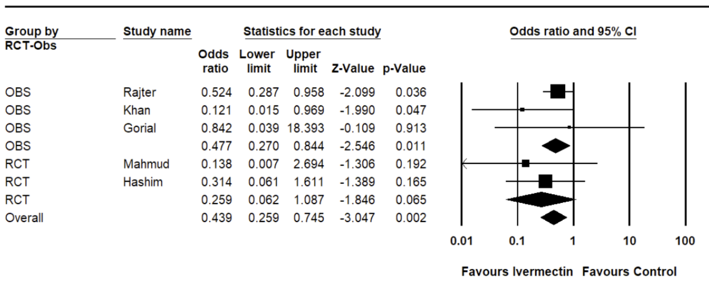
Figure 5. Metaanalysis of Ivermectin clinical studies
