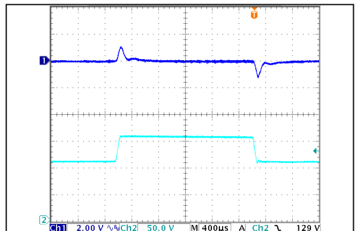
Figure 6: Output voltage response to step-change in input voltage (1V/ms). Load cap: 1 \mu F ceramic and 15 \mu F tantalum capacitors. Ch 1: V_{out} , Ch 2: V_{in} .
