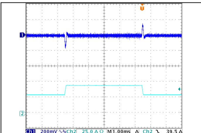
Figure 5: Output voltage response to step-change in load current (50%-75%-50% of I out (max); dI/dt = 0.1 A/μs). Load cap: 1 μF ceramic and 15 μF tantalum capacitors. Ch 1: V out , Ch 2: I out (25A/div)
